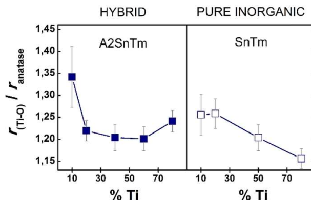
Fig. 3 Ti K-edge analysis for hybrid thin films A2SnTm (left side, solid symbols) and pure inorganic materials (right side, open symbols). The normalized Ti-O distance respect to anatase (up), r_{\text{Ti-O}}/r_{\text{anatase}} is plotted as a function of titania centers concentration. %Ti represents the fraction of Ti with respect to the total silica and titanium content expressed in percentage, ie. %Ti = T/(A + S + T)*100
